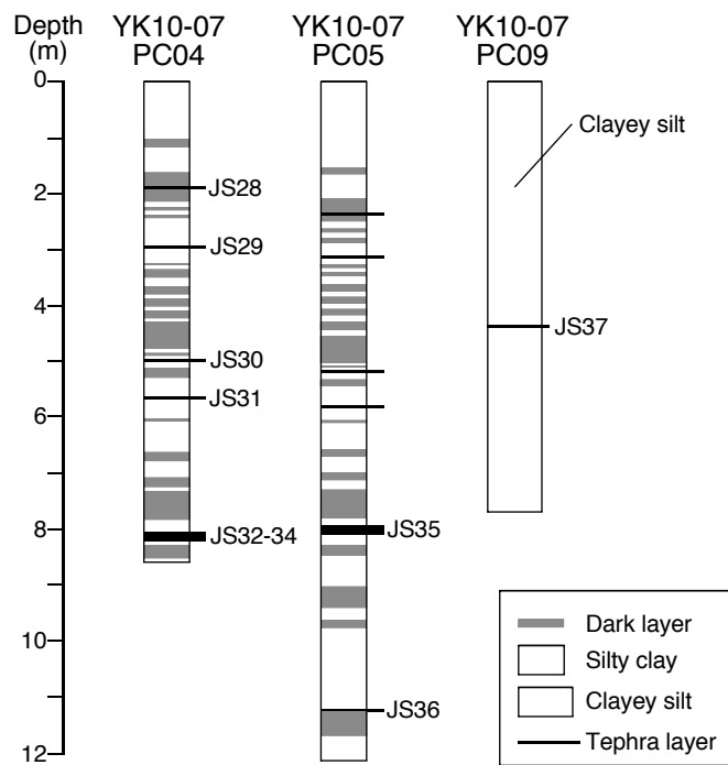
図S2 日本海中部の海底堆積物コア (YK10-07) の層序とテフラ試料 Fig.S2 Stratigraphical logs of the core samples (YK10-07) from central Japan Sea sediment cores and tephra samples.
